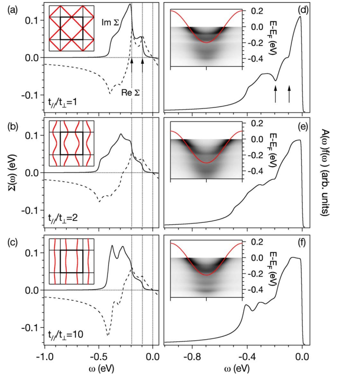
FIG. 4. (Color online) Spectral function calculations for a coupled electron-phonon system in a square lattice with different hopping anisotropies. (a)–(c) Electron self-energy calculated for a half-filled band coupled to two H_g phonons ( \omega_{ph}=0.195 and 0.096 eV, respectively). The hopping anisotropies are as follows: (a) t_{\parallel}/t_{\perp}=1 , isotropic dispersion, (b) t_{\parallel}/t_{\perp}=2 , and (c) t_{\parallel}/t_{\perp}=10 , highly anisotropic dispersion similar to the C_{60} chains. The insets show the corresponding Fermi surfaces [gray (red) line]. In the calculations we included the fivefold degeneracy of these C_{60} vibrational modes. (d)–(f) Occupied part of the interacting DOS convoluted with a Gaussian ( \sigma=10 meV) for the three different hopping anisotropies. The insets show calculated dispersion plots. A constant impurity scattering of 100 meV has been added for the plots of A(k, \omega) . The solid lines correspond to the noninteracting bands.
