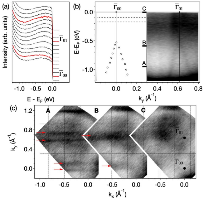
FIG. 2. (Color online) Angle-resolved photoemission data of C_{60} chains on Cu(553) measured at low temperature ( T=10 K). (a) Set of high-resolution EDCs measured along the chains. (b) Dispersion plot illustrating the electronic structure of C_{60}/Cu(553) in the direction along the chains. The dashed lines highlight the satellites from the nondispersing intramolecular phonons; the black circles follow the dispersion of the interface state in the HOMO-LUMO gap. (c) Constant energy maps at (a) -0.95 eV, (b) -0.6 eV, and (c) E_F . The C_{60} Brillouin zones are indicated by a dashed grid. Maximum intensity corresponds to black. k_y is oriented along [\bar{1}10] , the direction parallel to the chains. k_x is oriented along the perpendicular direction [\bar{3}\bar{3}10] .
