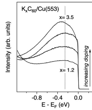
FIG. 3. K_x C_{60}/Cu(553) angle-integrated photoemission spectra measured for different doping levels of the LUMO ( T=10 K). The LUMO occupancy x was calibrated with the procedure described in Ref. 30. We found that in the undoped monolayer 1.2e/C_{60} are transferred from the substrate to the molecule.
