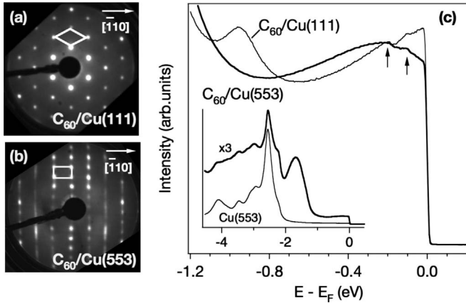
FIG. 1. (a) and (b) Low-energy electron diffraction (LEED) patterns of 1 ML C_{60}/Cu(111) and C_{60}/Cu(553) measured with 40 and 37 eV electron energy, respectively. The C_{60} chains on Cu(553) run along the [\bar{1}10] direction of the copper substrate. (c) Low-temperature ( T=10 K) He I\alpha angle-integrated photoemission spectra of one monolayer of C_{60} in a 1D and in a 2D molecular arrangement on Cu(553) and Cu(111) , respectively. The arrows mark the positions of the satellites due to electron-phonon coupling. The inset shows angle-integrated spectra of 1 ML C_{60}/Cu(553) and clean Cu(553) over a wider energy range.
